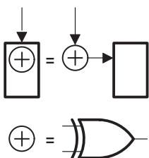
Figure 10. 18-Bit PSA/PRPG Configuration (10EA = 20EA = 1, 10EB = 20EB = 0)
