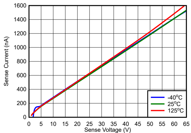
Figure 7-8. V_{\text{SENSE}} vs I_{\text{SENSE}}
