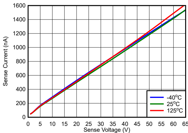
Figure 7-7. V_{\text{SENSE}} vs I_{\text{SENSE}}
