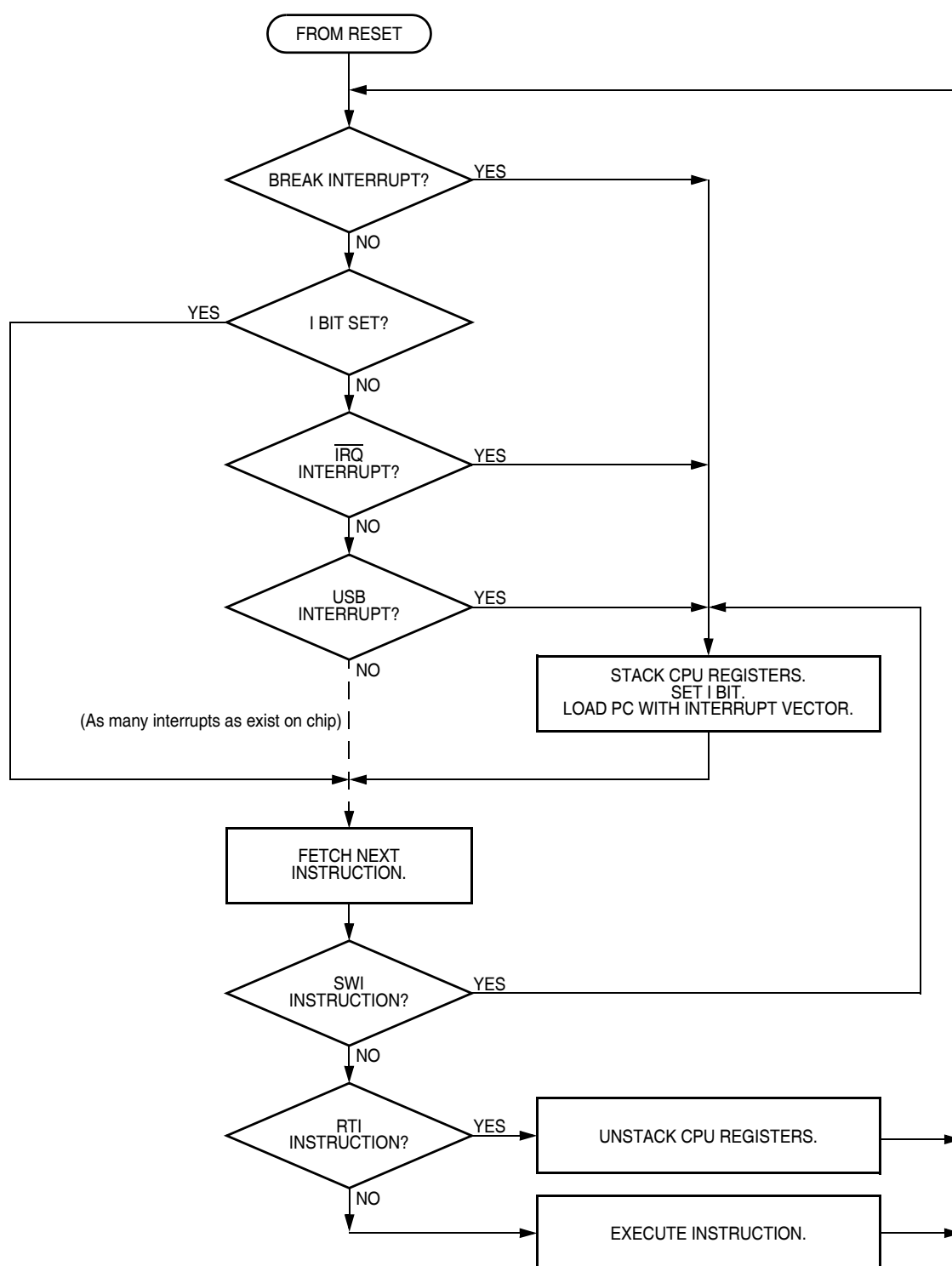
Figure 7-9. Interrupt Processing
