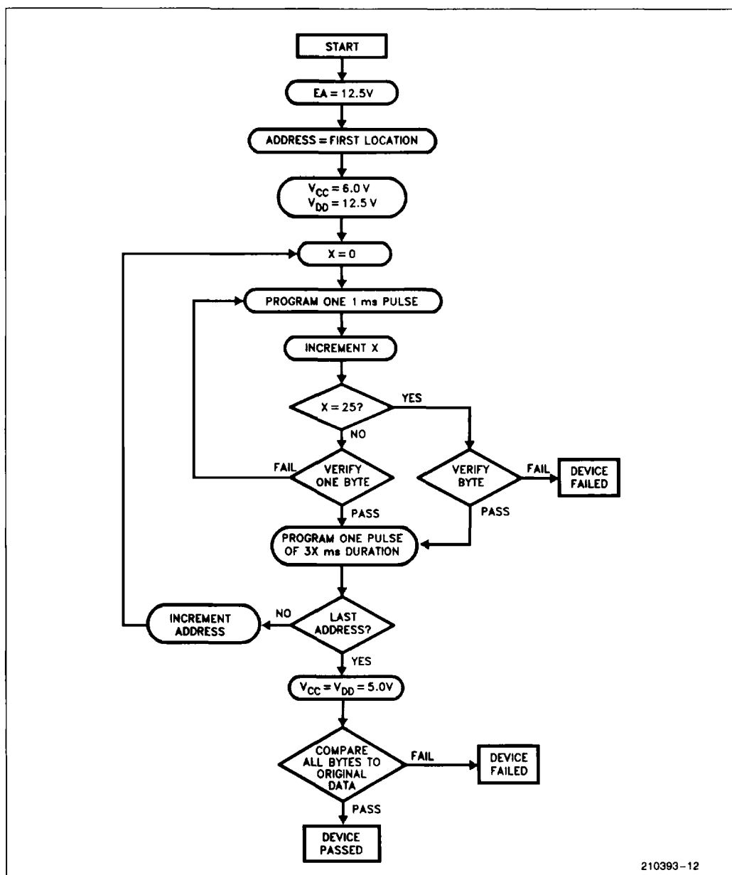
Figure 9. Programming Algorithm
