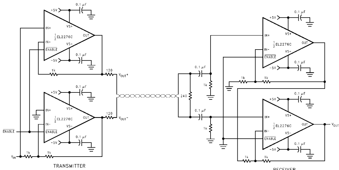
DIFFERENTIAL LINE-DRIVER/RECEIVER
