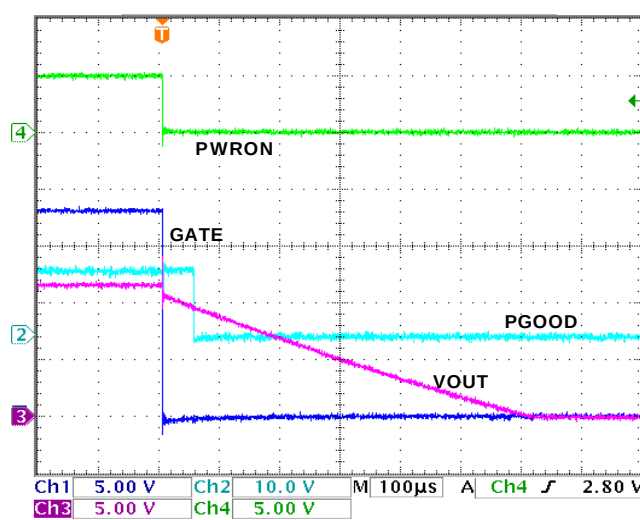
FIGURE 11. ISL6115A TURN-OFF
