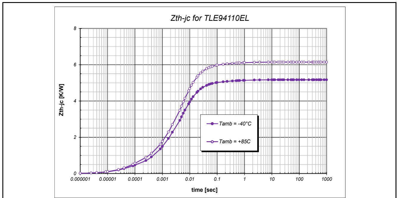
Figure 30 ZthJC Curve
