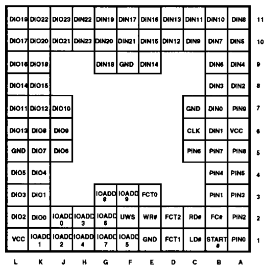
84 PIN GRID ARRAY BOTTOM VIEW
