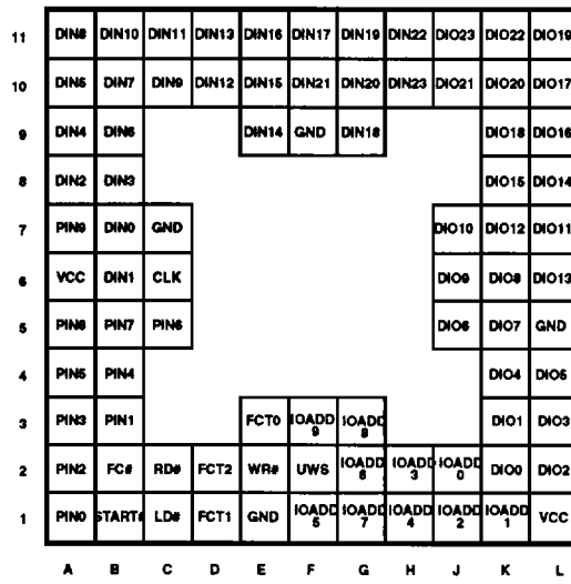
84 PIN GRID ARRAY TOP VIEW
