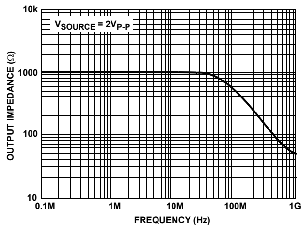
FIGURE 7. Z_{OUT} vs FREQUENCY - HiZ
