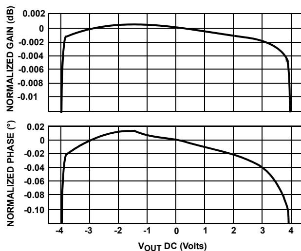
FIGURE 12. DIFFERENTIAL GAIN AND PHASE; V_{OUT} = 0.2V_{P-P} F_0 = 3.58\text{MHz} ; R_L = 500\Omega
