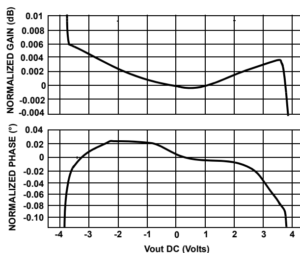
FIGURE 13. DIFFERENTIAL GAIN AND PHASE; V_{OUT} = 0.2V_{P-P} F_0 = 3.58\text{MHz} ; R_L = 150\Omega
