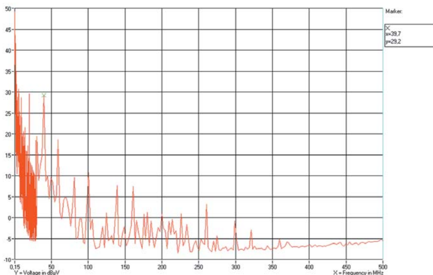
Graph 1: Emission IEC Norm 61967 part 4, MB90F394, FMOD=off.
