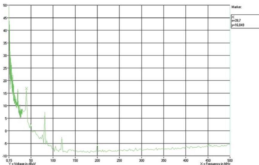
Graph 2: Emission IEC Norm 61967 part 4, MB90F394, FMOD=on.
