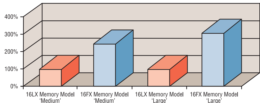
Graph 1 shows the performance ratio (Dhrystone 2.1) of 16FX compared to 16LX at 24MHz CPU frequency for different Memory Models. 16LX = 100%.
