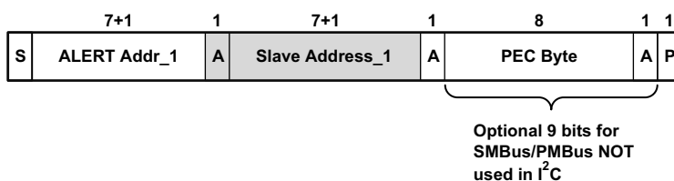
Figure 29. Alert Response Address (ARA, 0001_1001, 25h) for SMBus and PMBus, not used for I²C
