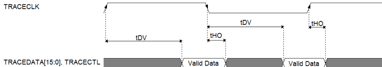
Figure 56. TRACE_CLKOUT specifications
