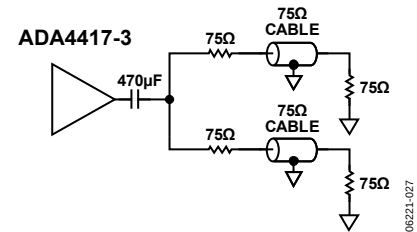
Figure 27. Driving Two AC-Coupled Loads with One Common Coupling Capacitor
