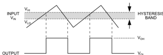
Figure 8: Analog Comparator Hysteresis Band and Output Switching Points.
