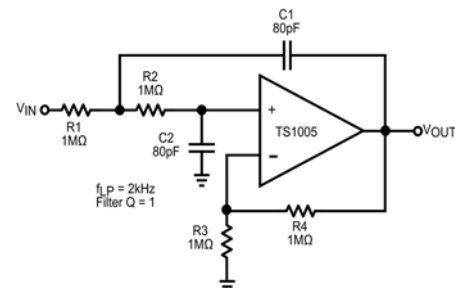
Figure 3: A Micropower 2-Pole Sallen-Key Low-Pass Filter.
