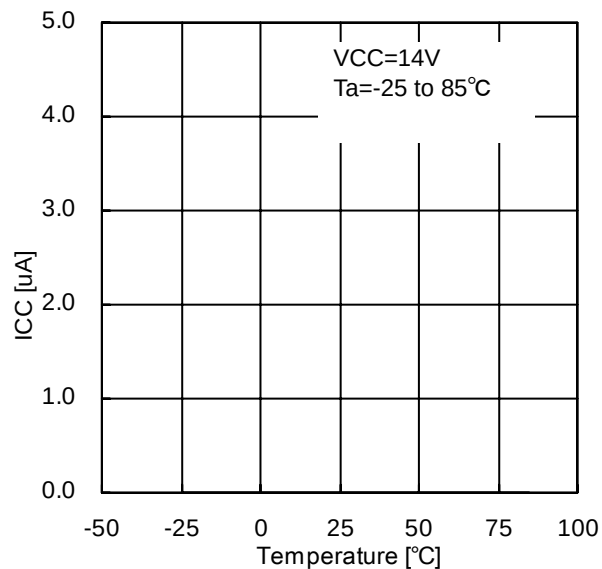
Figure.11 ICC(OFF) - Ta
