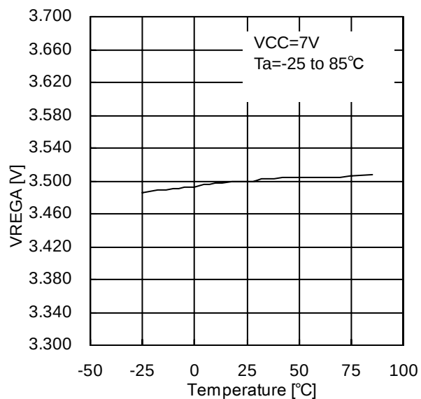
Figure.15 VREGA – Ta
