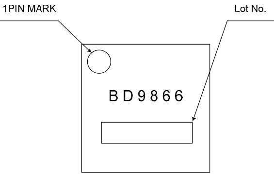
Figure. 65 Marking diagram
