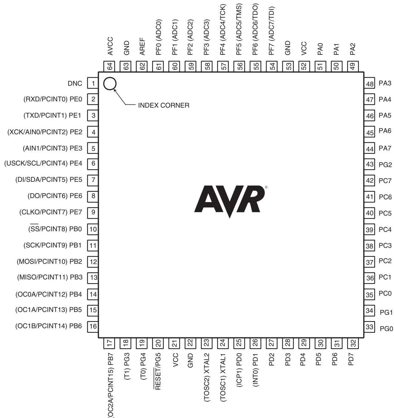
Figure 1-1. Pinout ATmega165P
