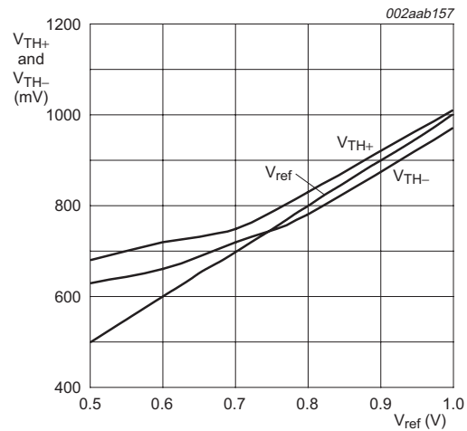
Fig 5. GTL V_{TH+} and V_{TH-} versus V_{ref} ; T_{amb} = +25^\circ\text{C}
