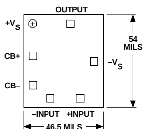
Chip Layout
