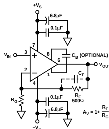
Figure 3. Noninverting Gain Connection Diagram
