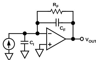
Figure 1. Transimpedance Configuration
