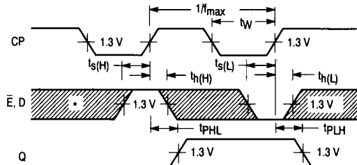
Figure 2. Clock to Output Delays Clock Pulse Width, Frequency, Setup and Hold Times Data or Enable to Clock
