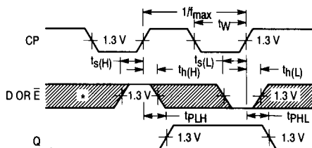
SN54/74LS377
