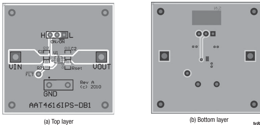
Figure 18. AAT4616IPS Evaluation Board Layer Details
