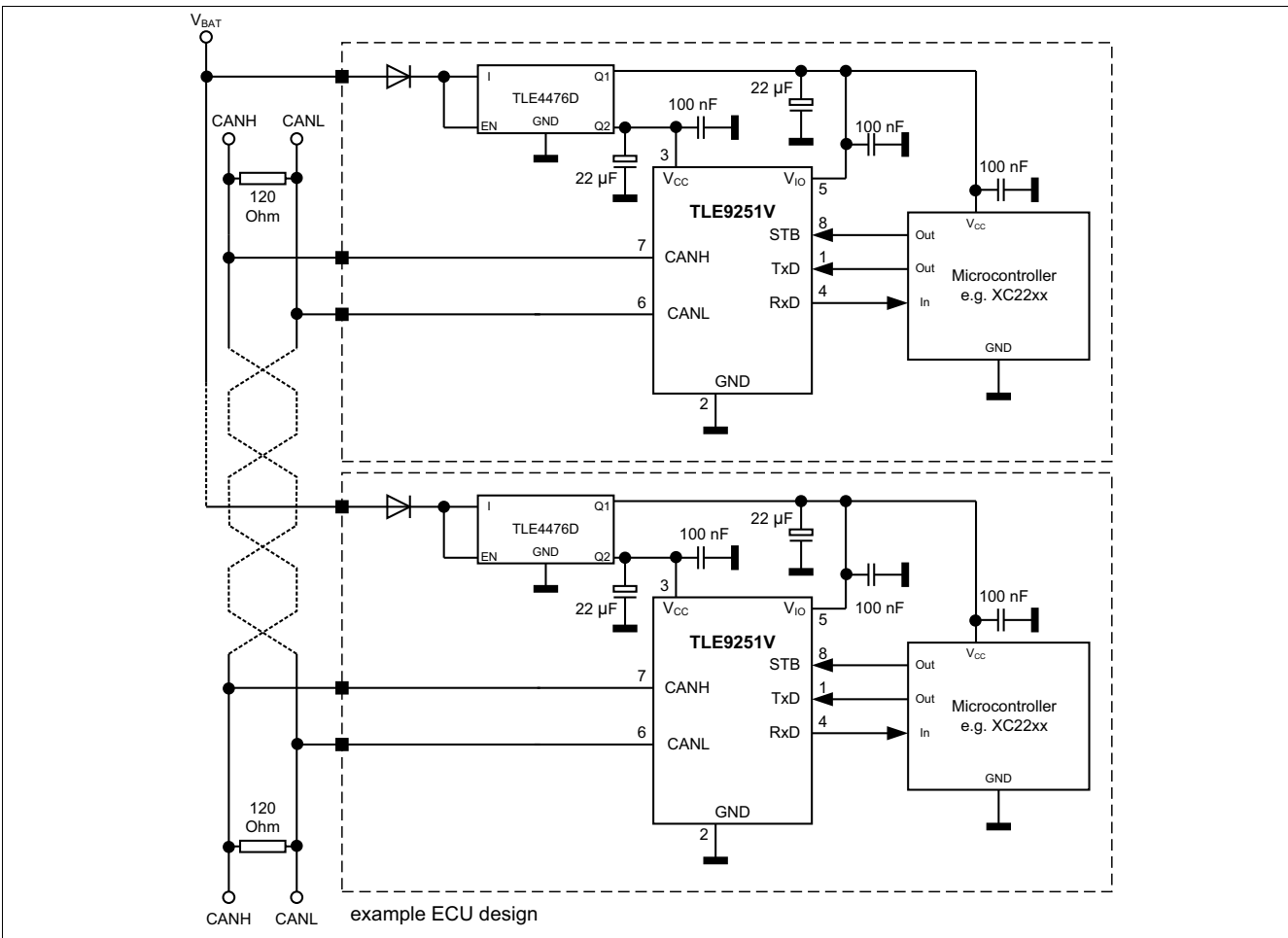
Figure 18 Application circuit
