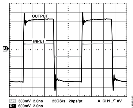
Figure 30. Large Signal Pulse Response, V_{OUT} = 4 V p-p, V_S = 3.3 V
