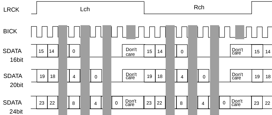
Figure 12. Mode 2 Timing
