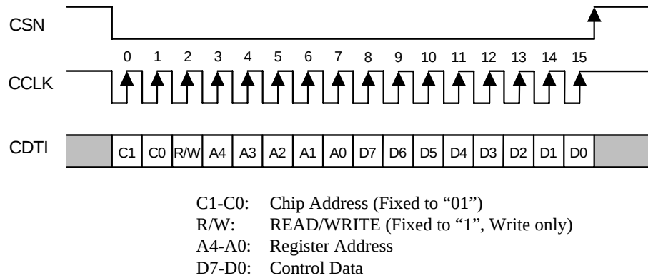
Figure 21. 3-wire Serial Control I/F Timing
