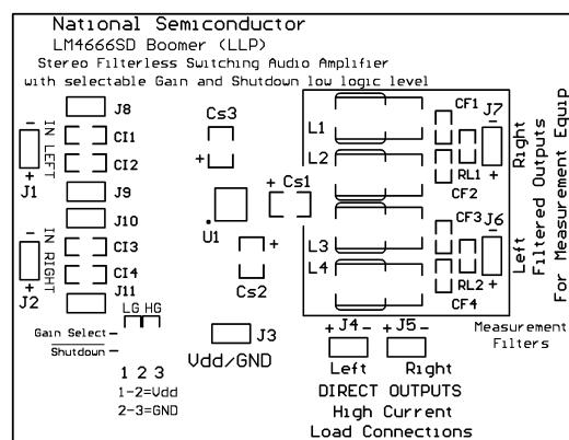
Silk Screen
