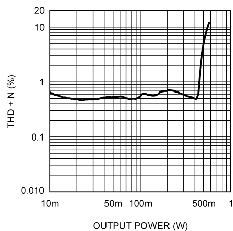
THD+N vs Output Power/Channel V_{DD} = 3V , R_L = 15\mu H + 8\Omega + 15\mu H f = 1kHz, 22kHz BW
