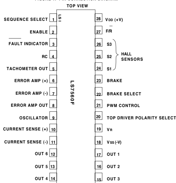
FIGURE 1. PIN CONNECTION DIAGRAM
