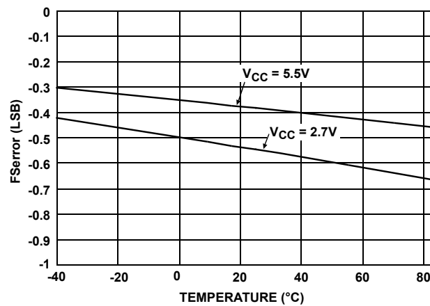
FIGURE 6. FSerror vs TEMPERATURE
