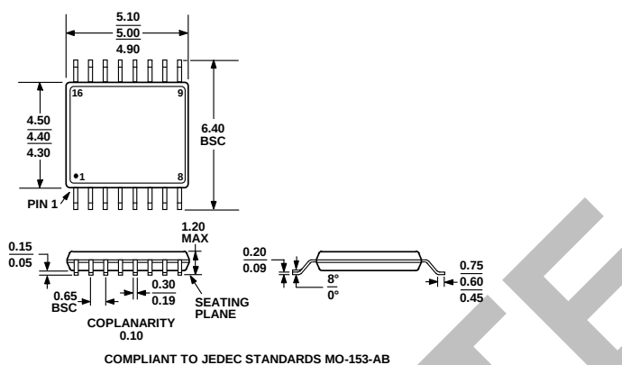
Figure 20. 16-Lead Thin Shrink Small Outline Package [TSSOP] (RU-16) Dimensions shown in millimeters
