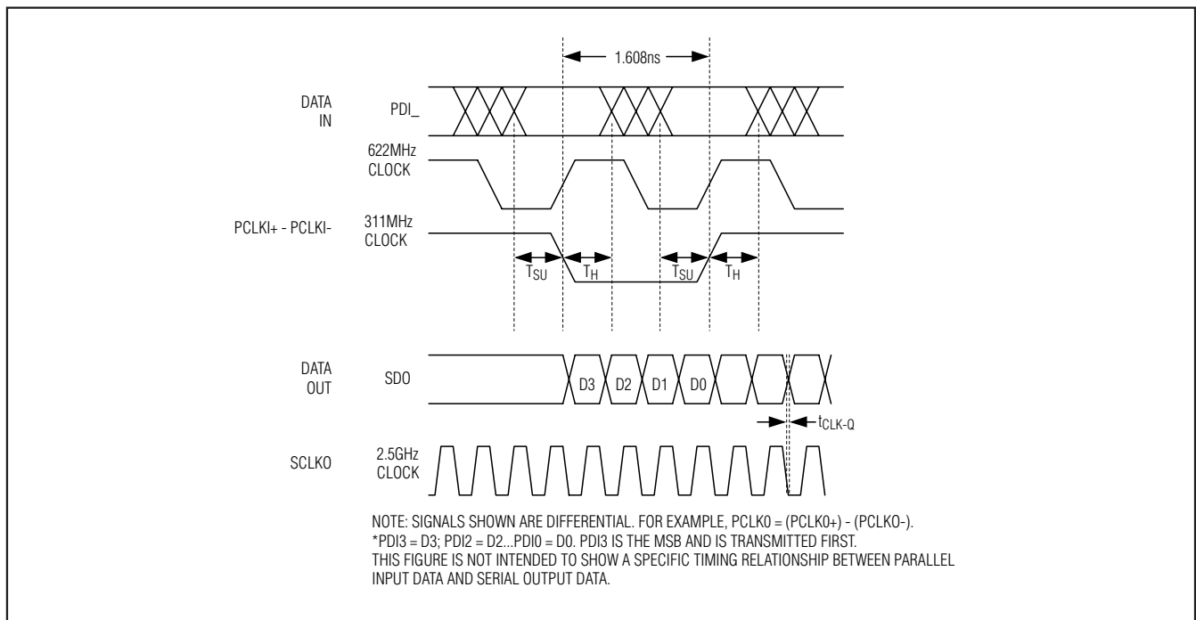
Figure 1. Timing Diagram
