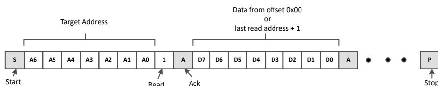
Figure 8-12. I2C Read Without Repeated Start
