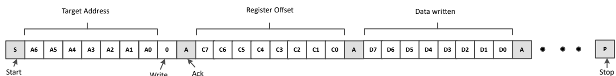
Figure 8-11. I 2 C Write with Data
