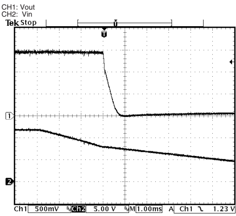
POWER-DOWN, 40A LOAD
