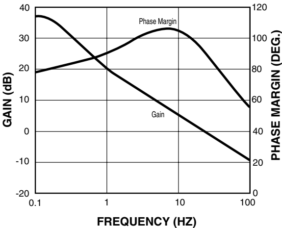
CLOSED LOOP RESPONSE
