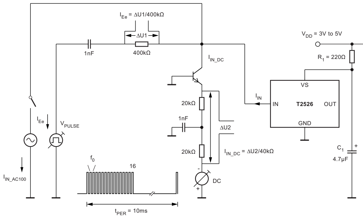
Figure 6-9. Test Circuit
