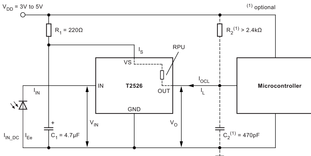
Figure 6-10. Application Circuit
