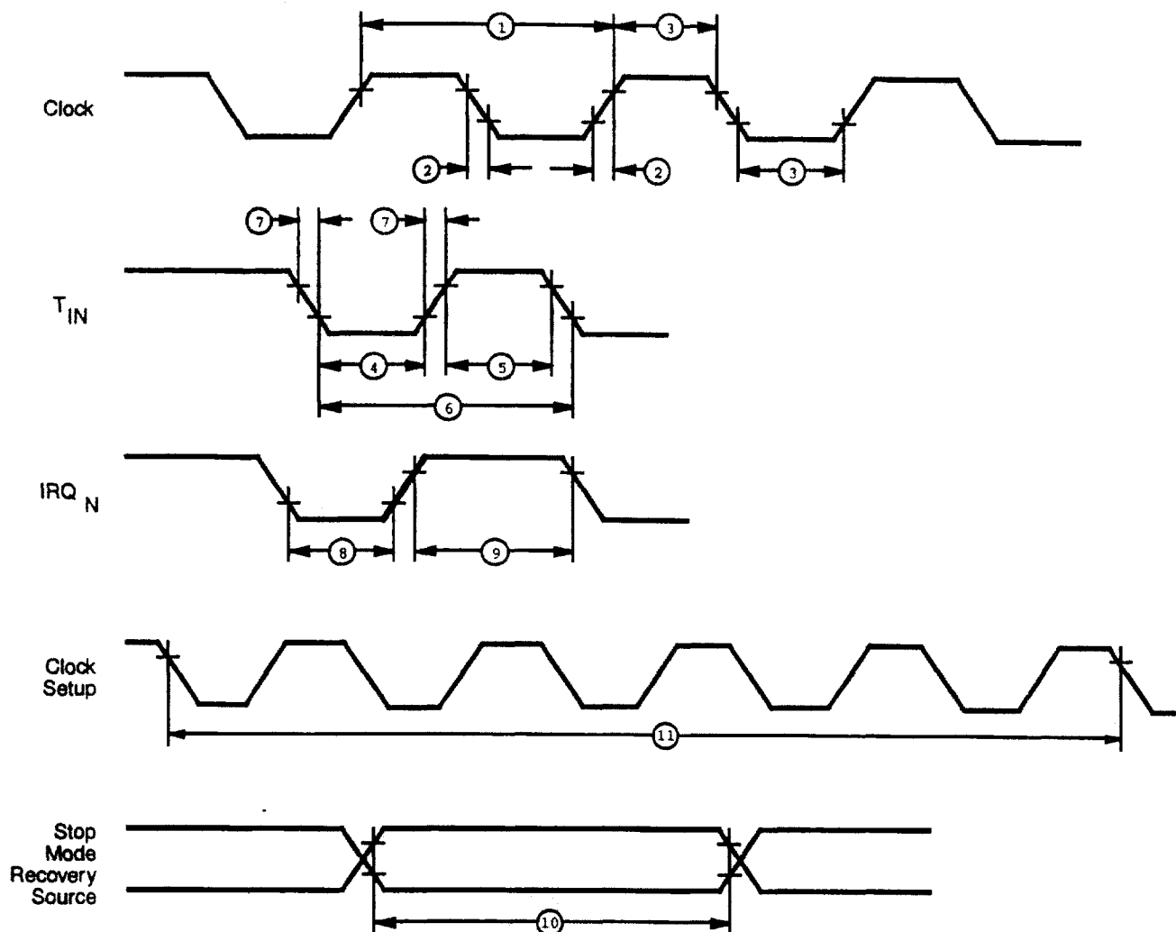
Figure 8. Additional Timing
