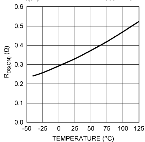
SOT23 R_{DS(ON)} vs Temperature ( V_{BOOST} - V_{SW} = 3V )
