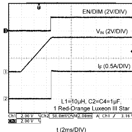
FIGURE 7. Startup Response to V_{IN} with EN/DIM delayed
