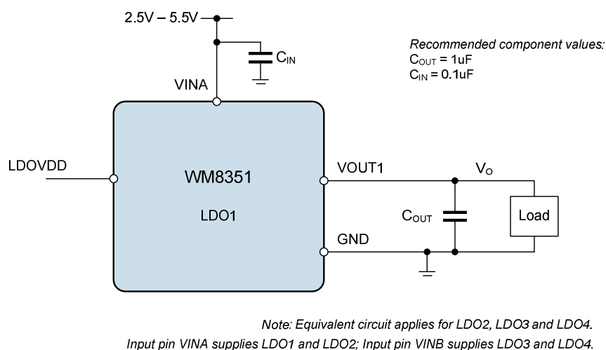
Figure 71 LDO Regulator Connections
