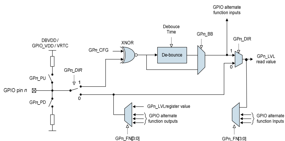
Figure 79 GPIO Equivalent Circuit
