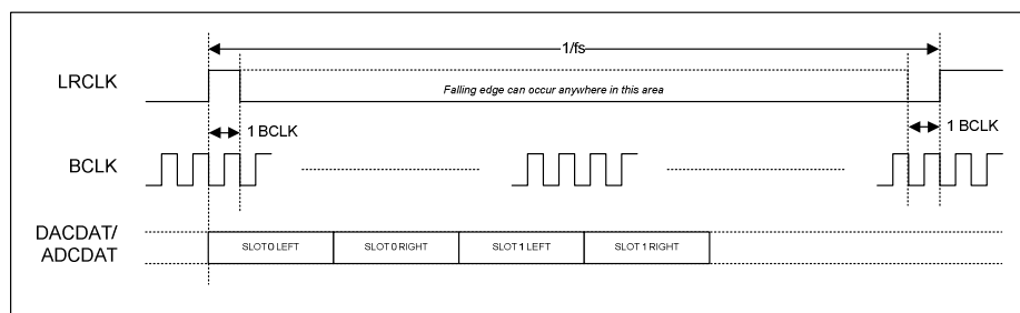
Figure 61 DSP/PCM Mode B, Slave Mode, with TDM
