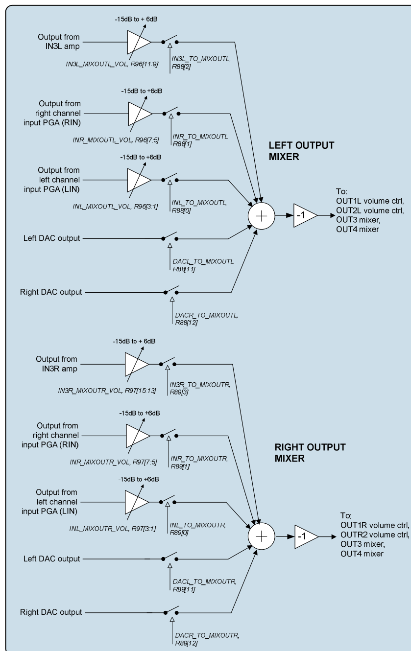
Figure 43 Output Mixers
