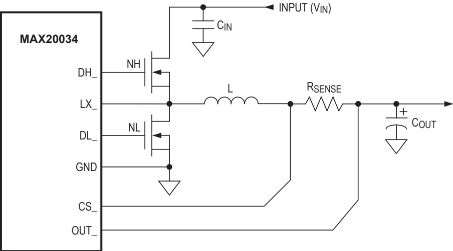
A) OUTPUT SERIES-RESISTOR SENSING
