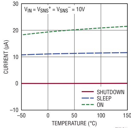
SNS^+ Supply Current vs Temperature
