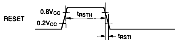
Figure 60 Reset Timing
