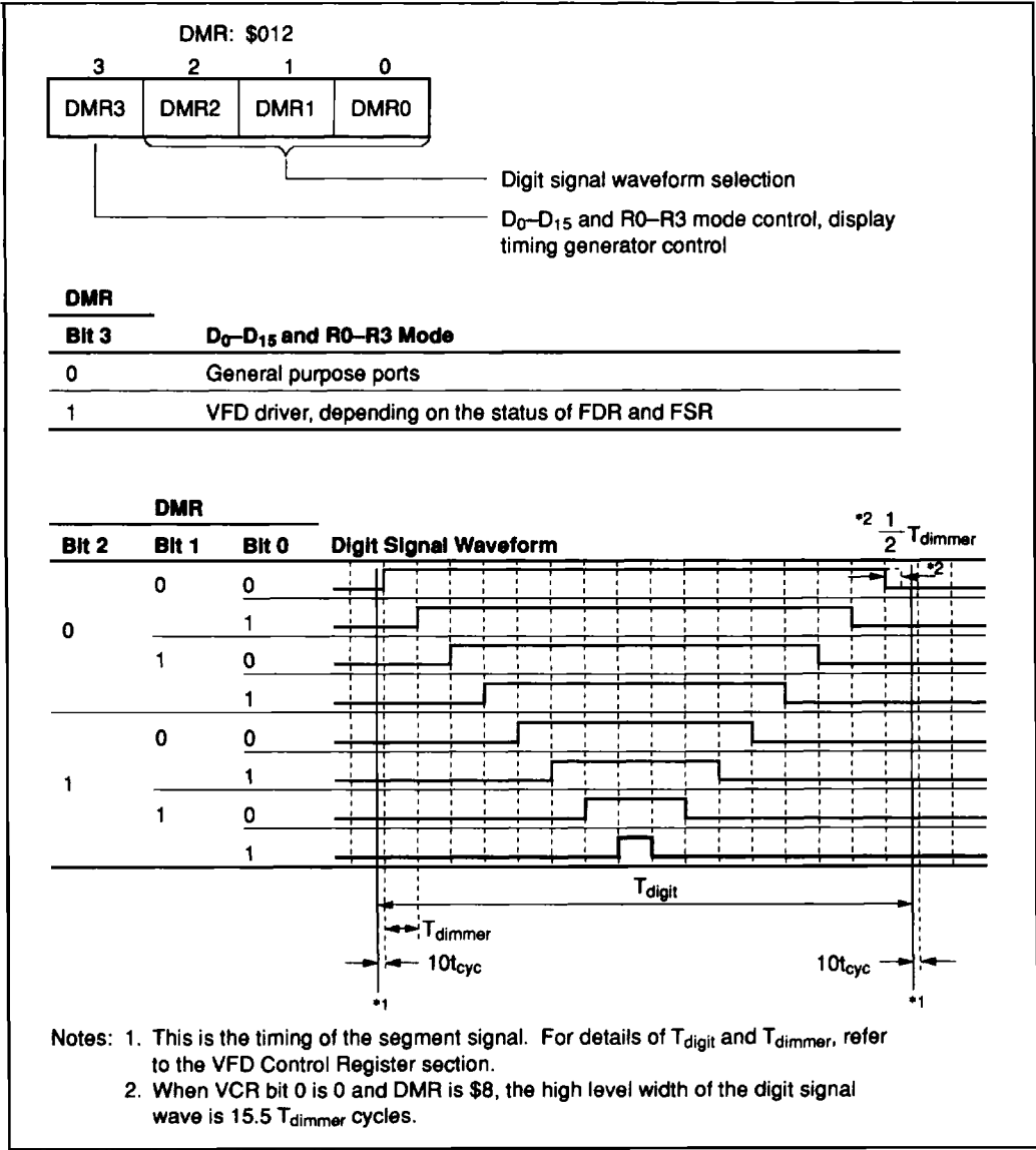
Figure 45 Dimmer Mode Register
