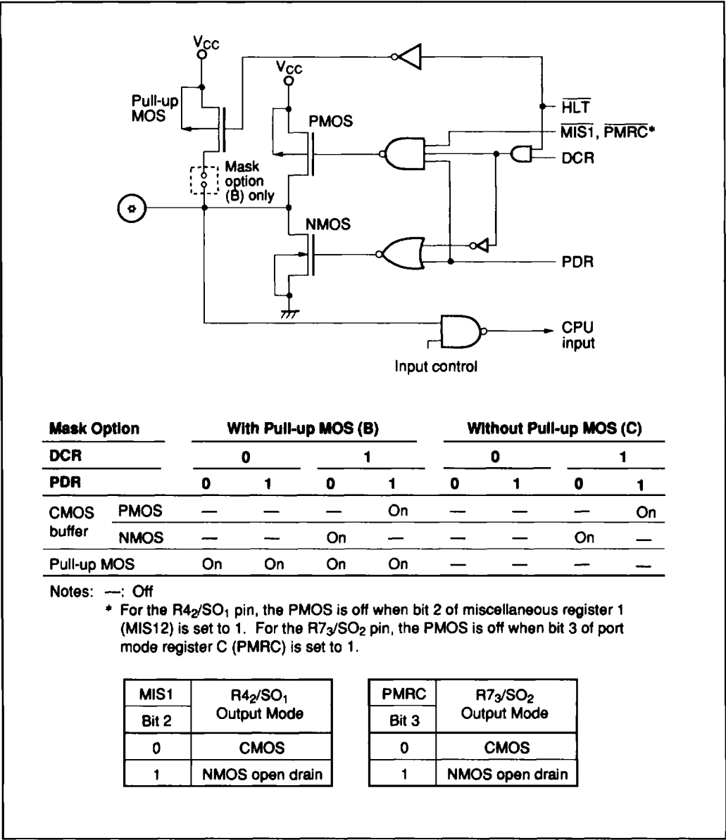
Figure 24 Input/Output Buffer
