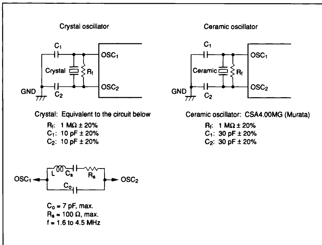
Figure 56 Oscillation Circuits (1)
