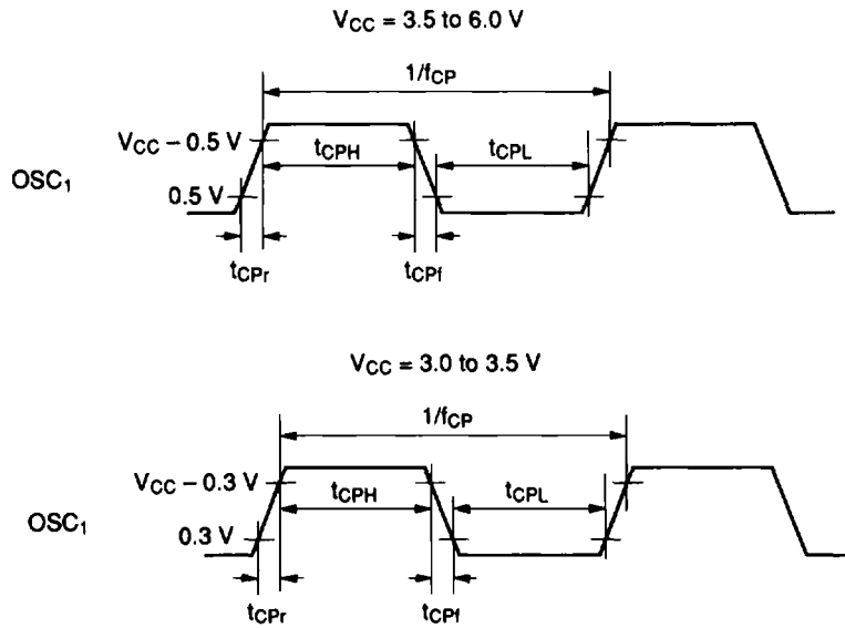
Figure 58 Oscillator Timing
