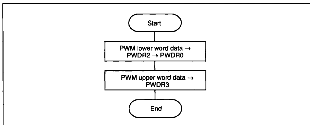
Figure 48 PWM Operation
