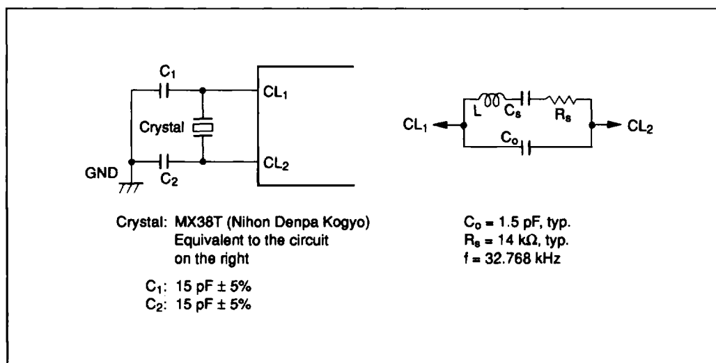
Figure 57 Oscillation Circuits (2)
