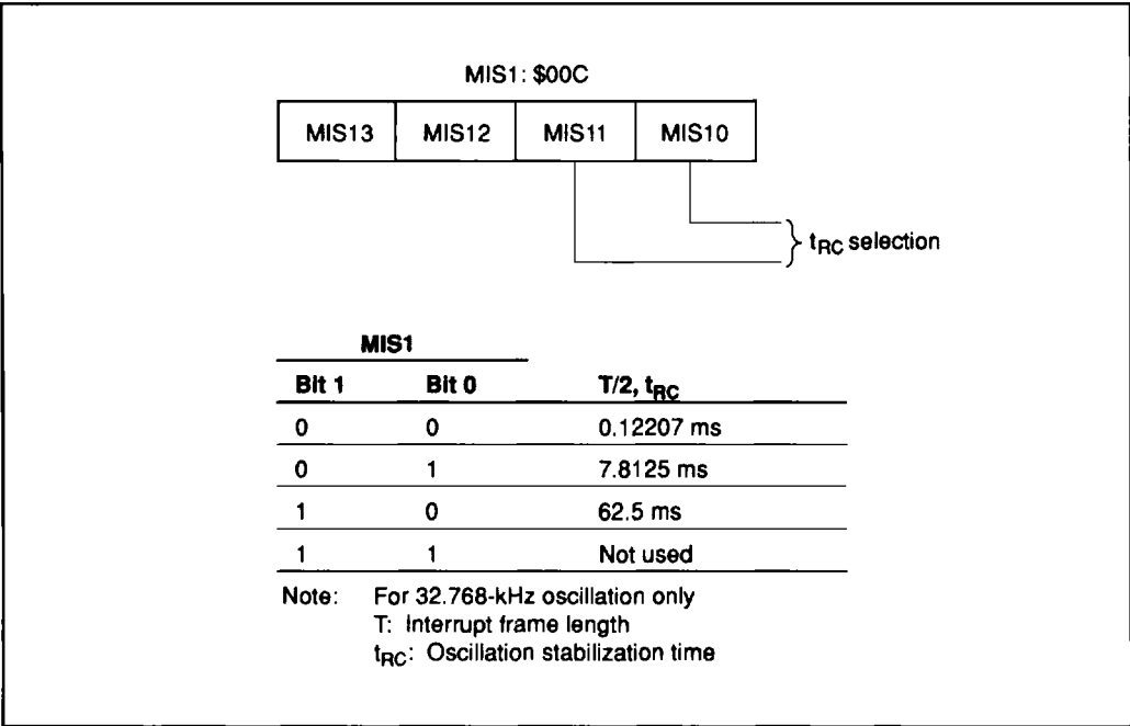
Figure 18 Miscellaneous Register 1
