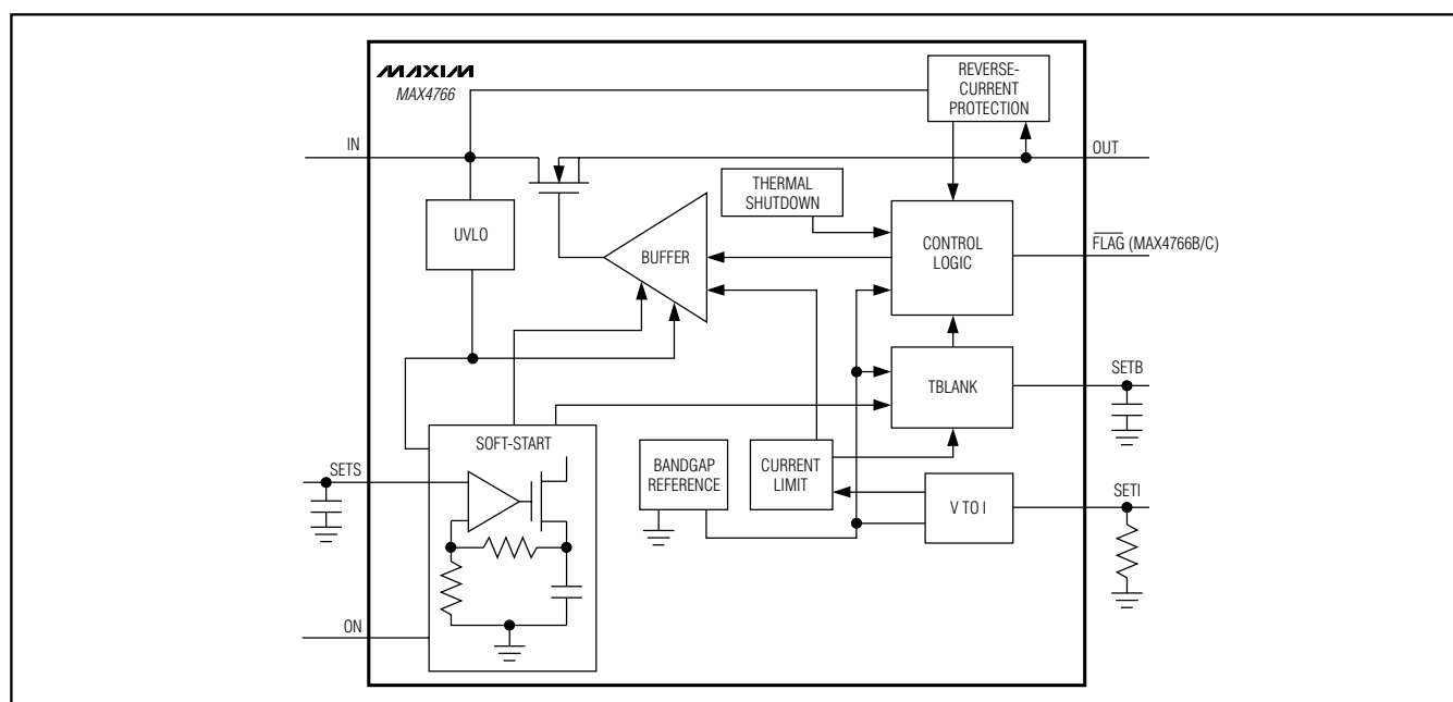
Figure 1. Functional Diagram
