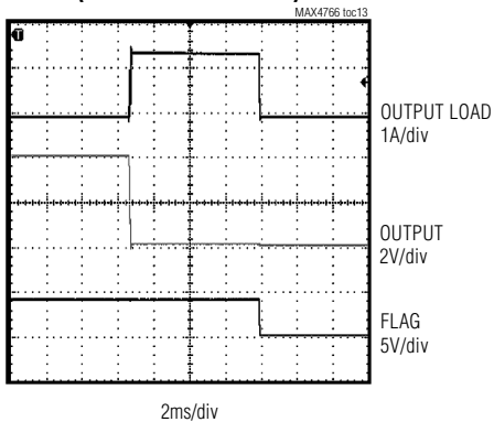
FLAG RESPONSE TIME (OVERLOAD CONDITION)
