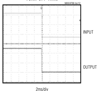
TURN-OFF TIME
