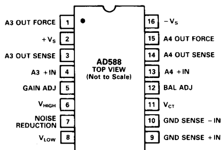
D Package
