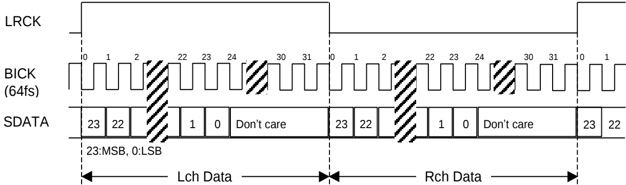
Figure 13. Mode 2 Timing
