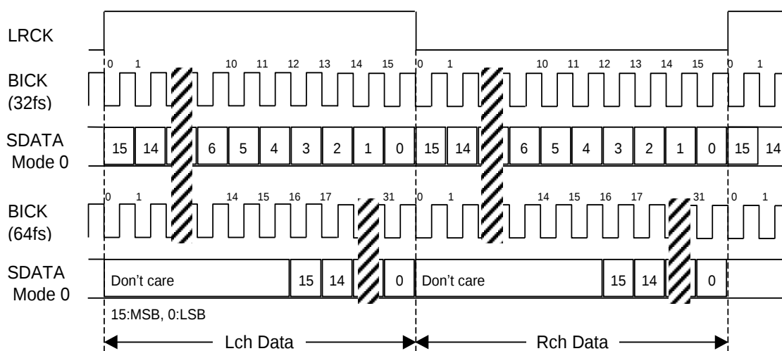
Figure 11. Mode 0 Timing
