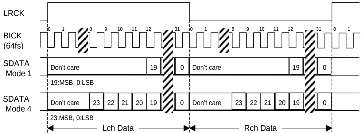
Figure 12. Mode 1/4 Timing
