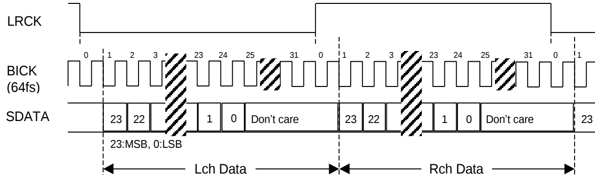
Figure 14. Mode 3 Timing
