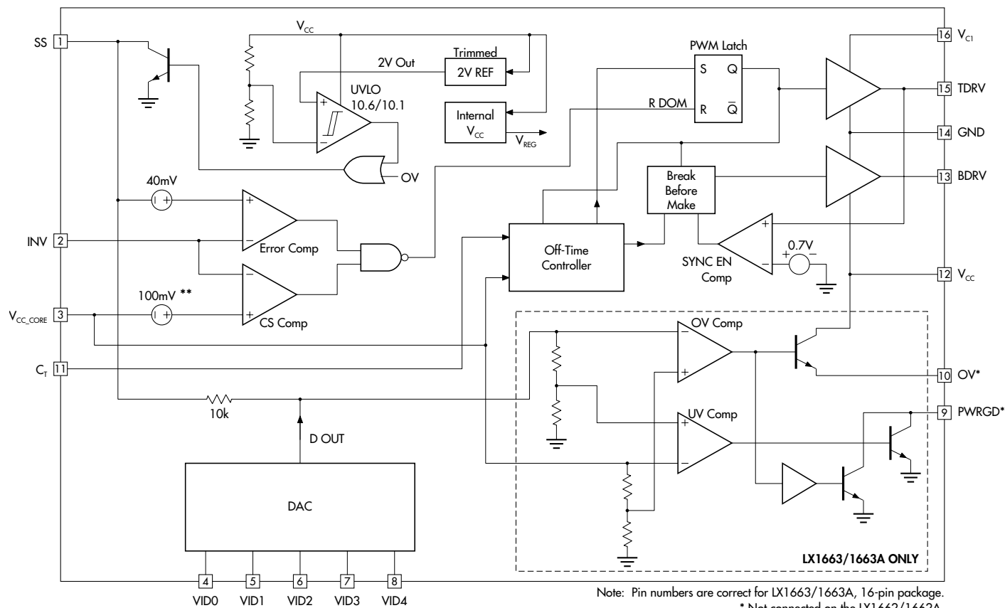
FIGURE 5 — Block Diagram
