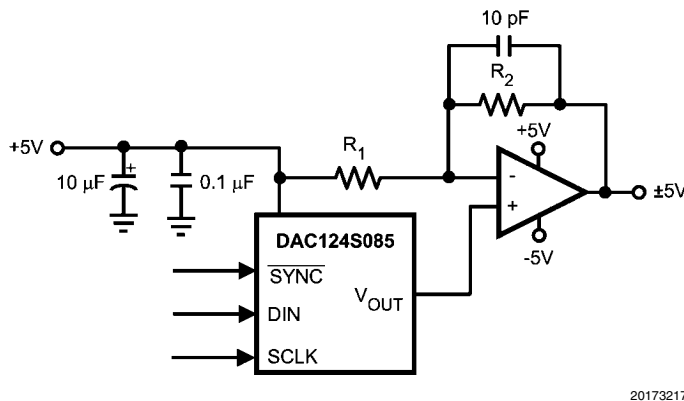
FIGURE 9. Bipolar Operation
