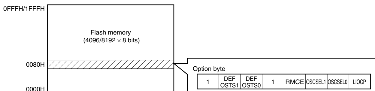
Figure 18-1. Positioning of Option Byte
