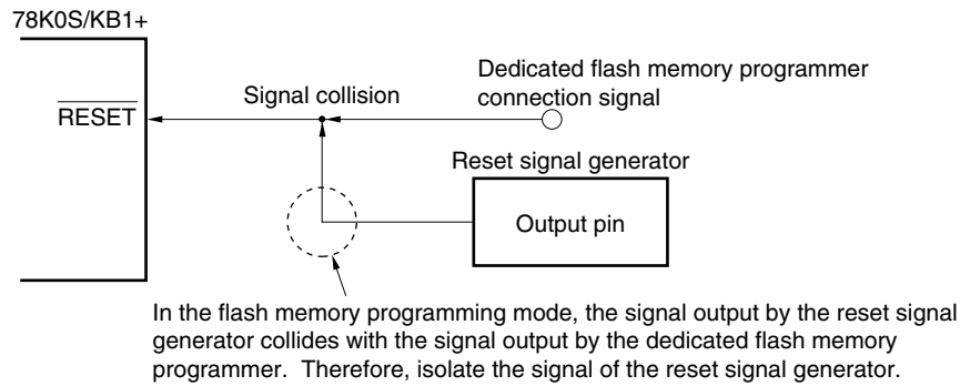
Figure 19-6. Signal Collision (RESET Pin)
