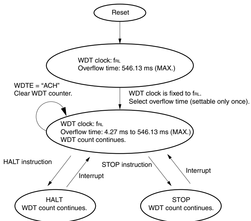
Figure 9-4. Status Transition Diagram When “Low-Speed Internal Oscillator Cannot Be Stopped” Is Selected by Option Byte
