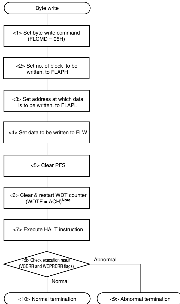
Figure 19-22. Example of Byte Write Operation in Self Programming Mode
