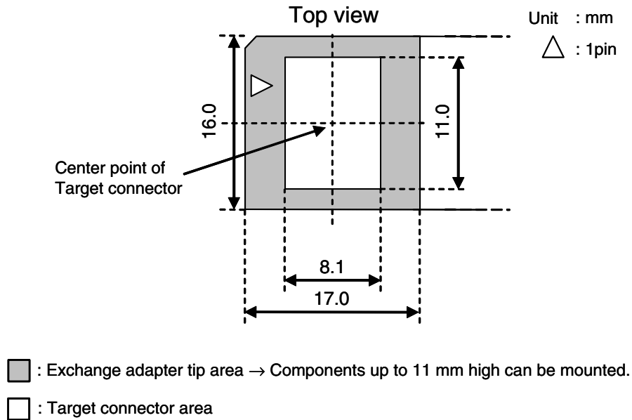
Figure B-1. When using the 78K0S/Kx1+ emulation probe (For 30-Pin MC Package)
