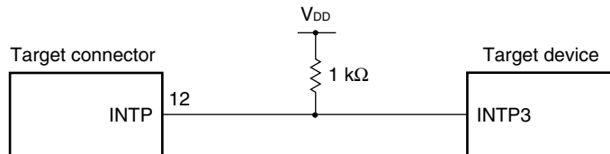
Figure 20-2. Circuit Connection for the Case Where INTP3 Pin Is Not Used in Target System
