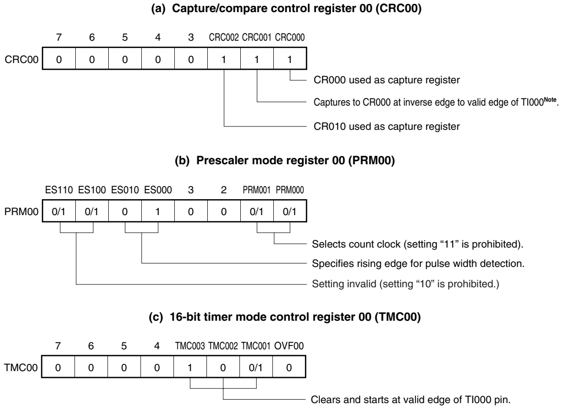
Figure 6-25. Control Register Settings for Pulse Width Measurement by Means of Restart (with Rising Edge Specified)
