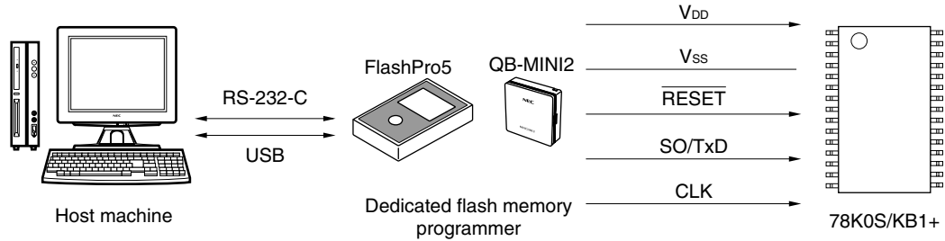
Figure 19-2. Environment for Writing Program to Flash Memory (FlashPro5/QB-MINI2)
