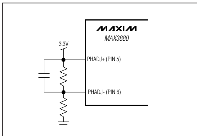
Figure 6. Phase-Adjust Resistor-Divider
