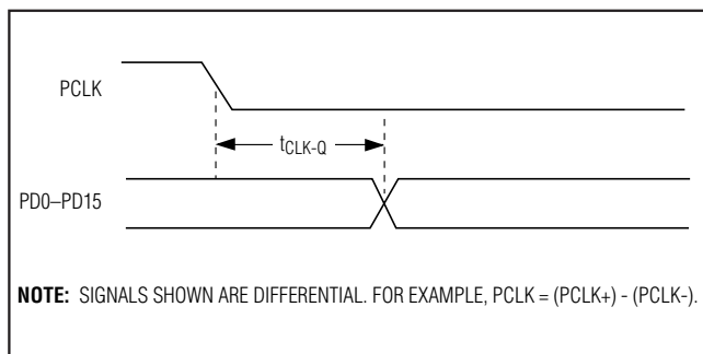
Figure 5. Timing Parameters
