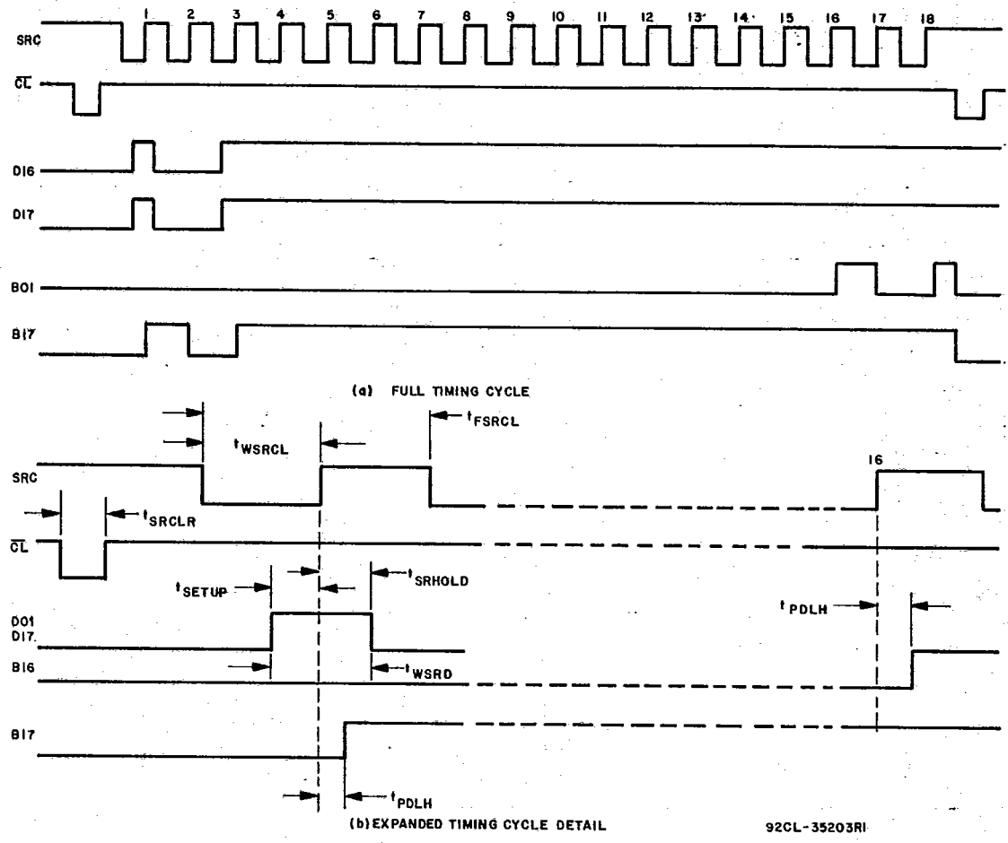
Fig. 2 - Functional timing diagram-shift registers function.
