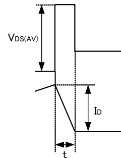
Figure 13-3. Waveform at Avalanche Breakdown
