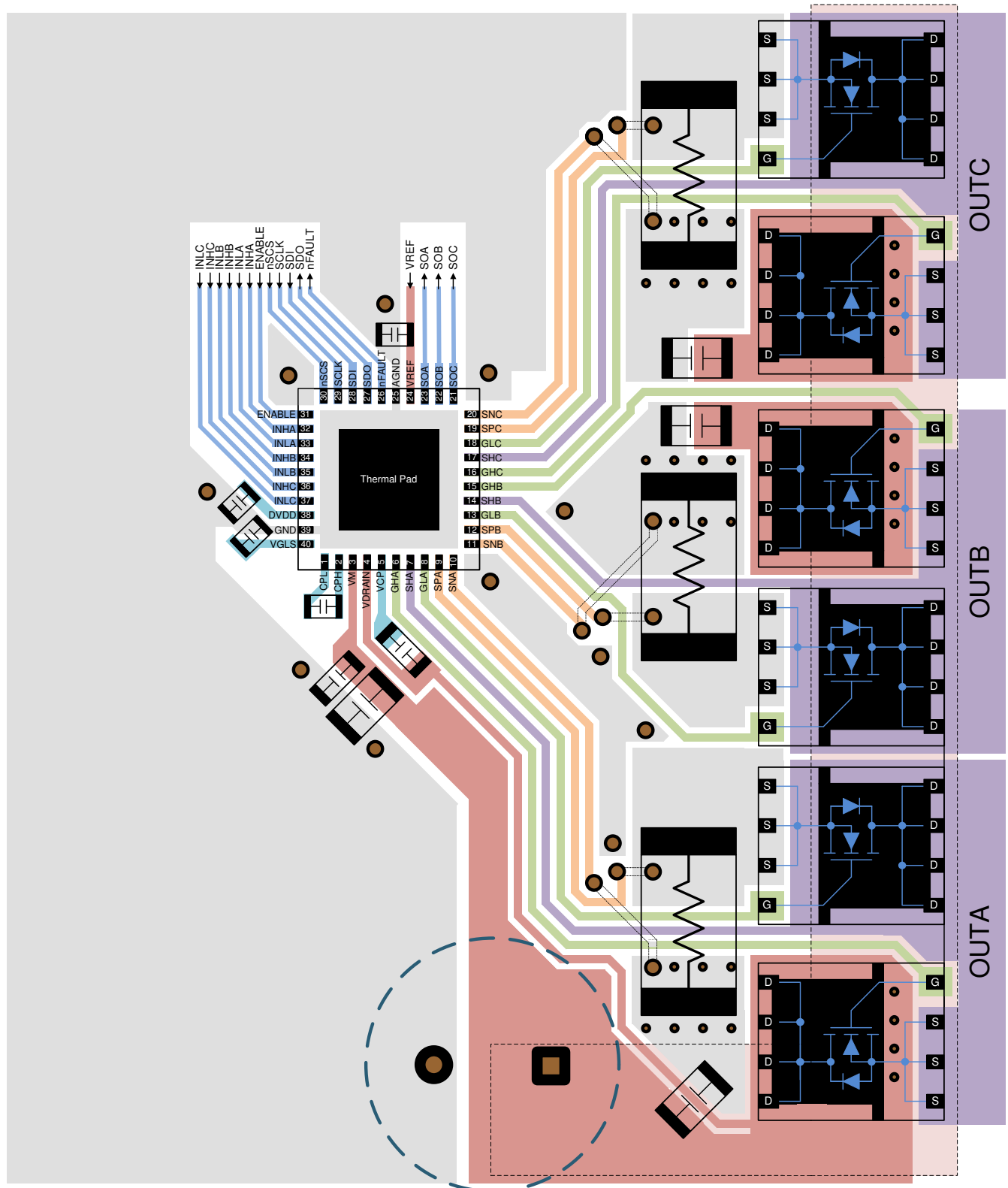
Figure 11-1. Layout Example
