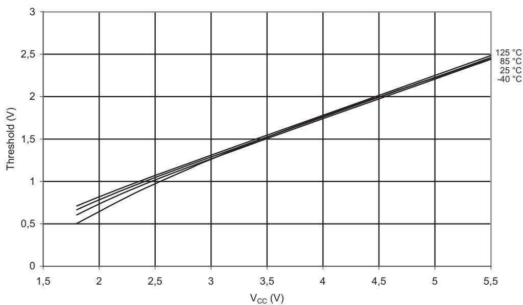
Figure 2-31. V_{IH}-V_{IL} : Input Hysteresis vs. V_{CC} (I/O Pin)
