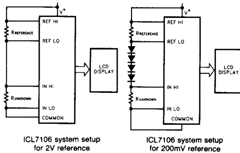
Figure 22. Ratiometric Ohms Measurement
