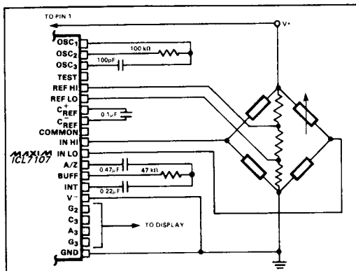
Figure 15. ICL7107 Measuring Ratiometric Values of a Load Cell. Desired Sensitivity is Determined by Resistor Values Within the Bridge.
