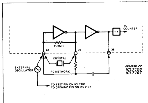
Figure 7. Clock Circuits
