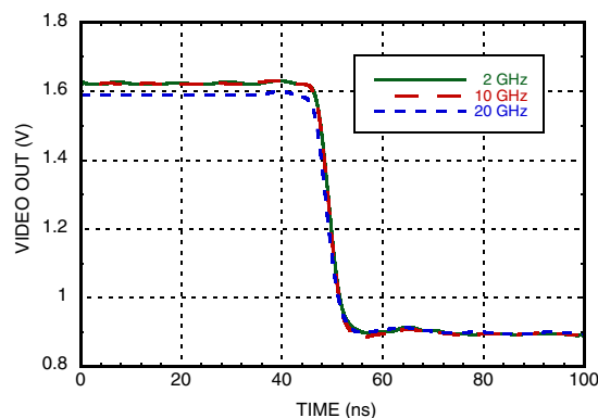
Fall Time for Various Frequencies @ P_{in} = 0 \text{ dBm} [1]
