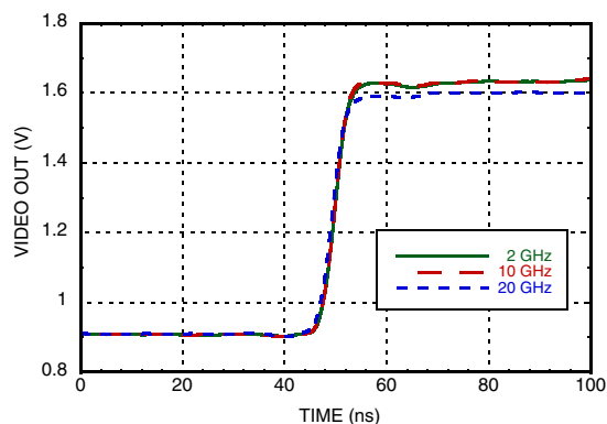
Rise Time for Various Frequencies @ P_{in} = 0 \text{ dBm} [1]
